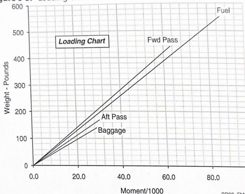
Figure 6-3: Loading Chart
